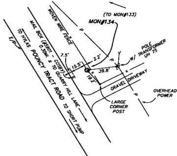
MONUMENT RECOVERY SITE SKETCH (NO SCALE)
