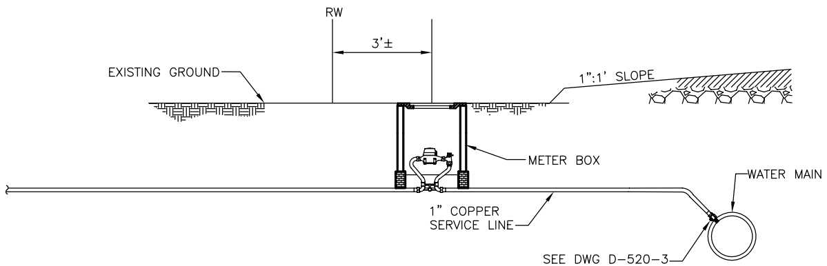
TYPICAL DPW ROAD SECTION WITHOUT CURB AND GUTTER
