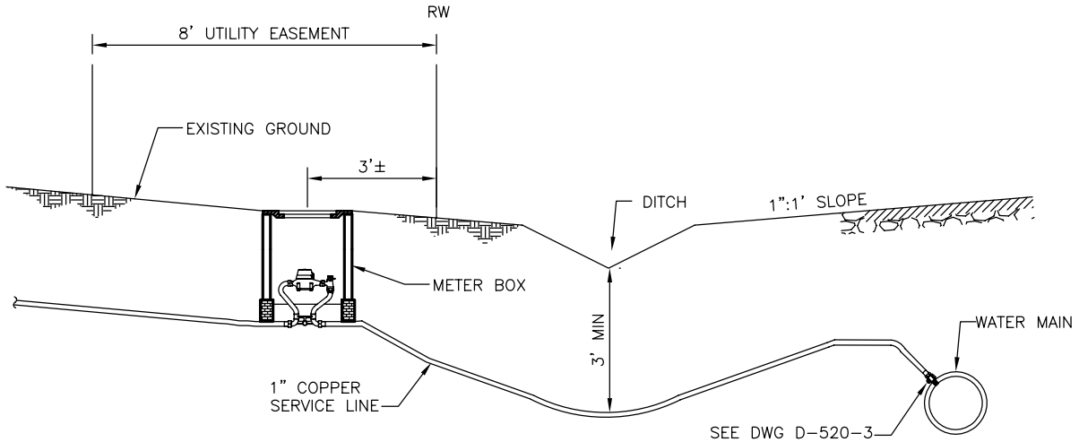
TYPICAL DPW ROAD SECTION WITHOUT CURB AND GUTTER WITH DITCH
