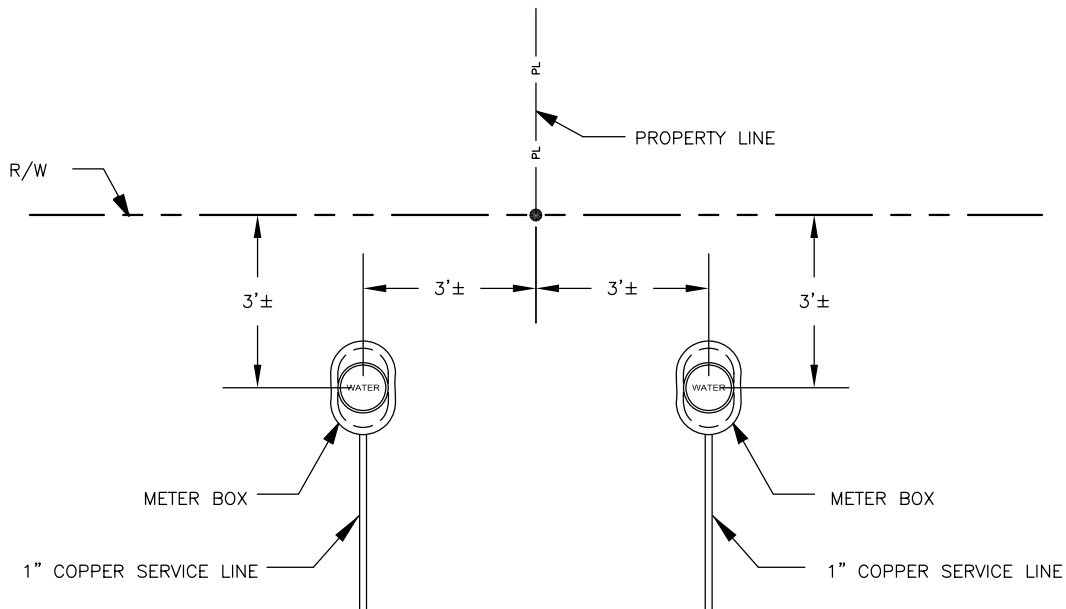
LOCATION OF METER BOXES PLACED INSIDE THE R/W
