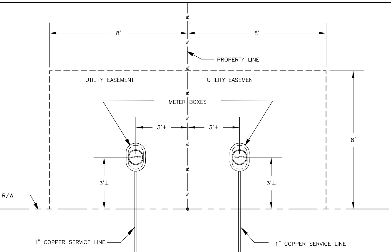
LOCATION OF METER BOXES PLACED OUTSIDE THE R/W
