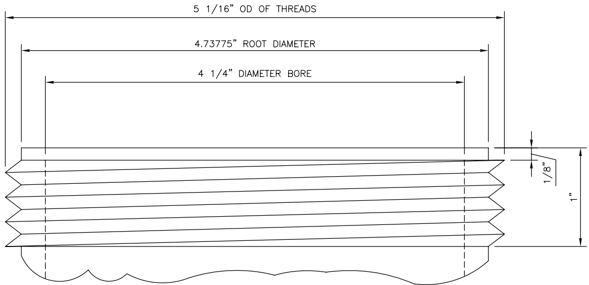
4 1/4" PUMPER NOZZLE NUMBER PER HYDRANT: 1
