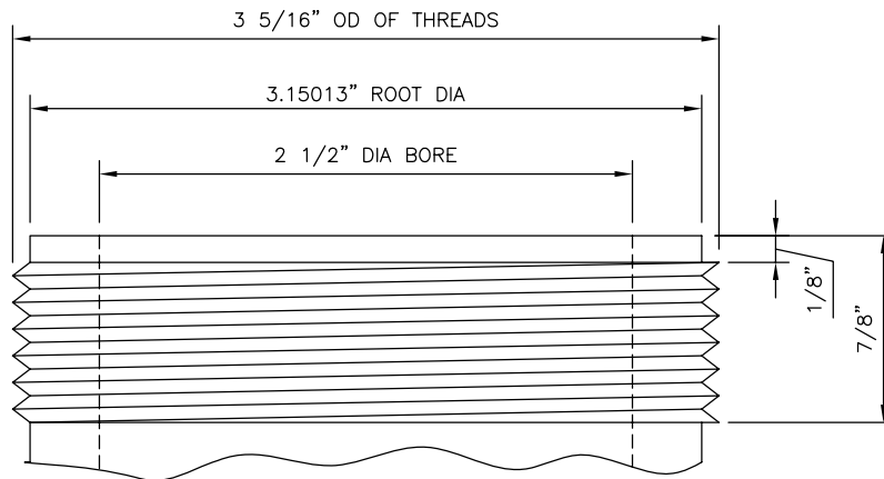
2 1/2" HOSE NOZZLE NUMBER PER HYDRANT: 2
