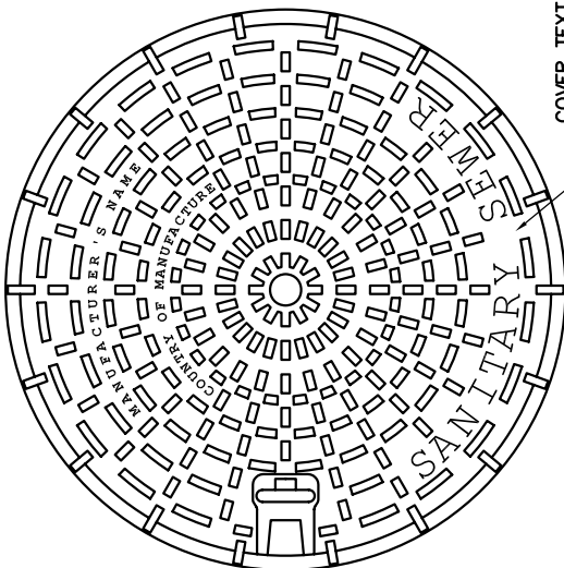
TOP OF COVER
